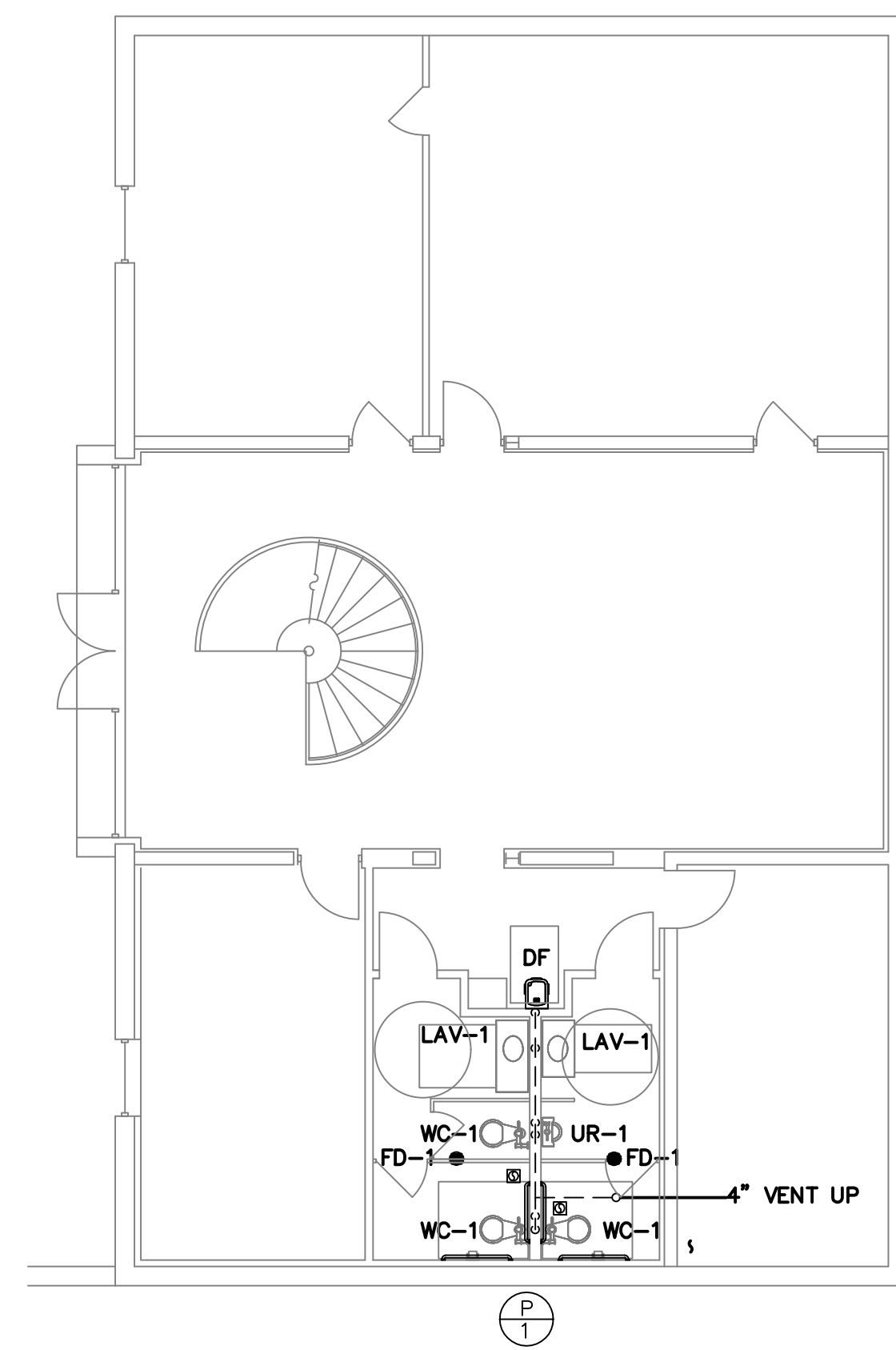
LOWER LEVEL WASTE FLOOR PLAN SCALE: 1/8" = 1'-0"
