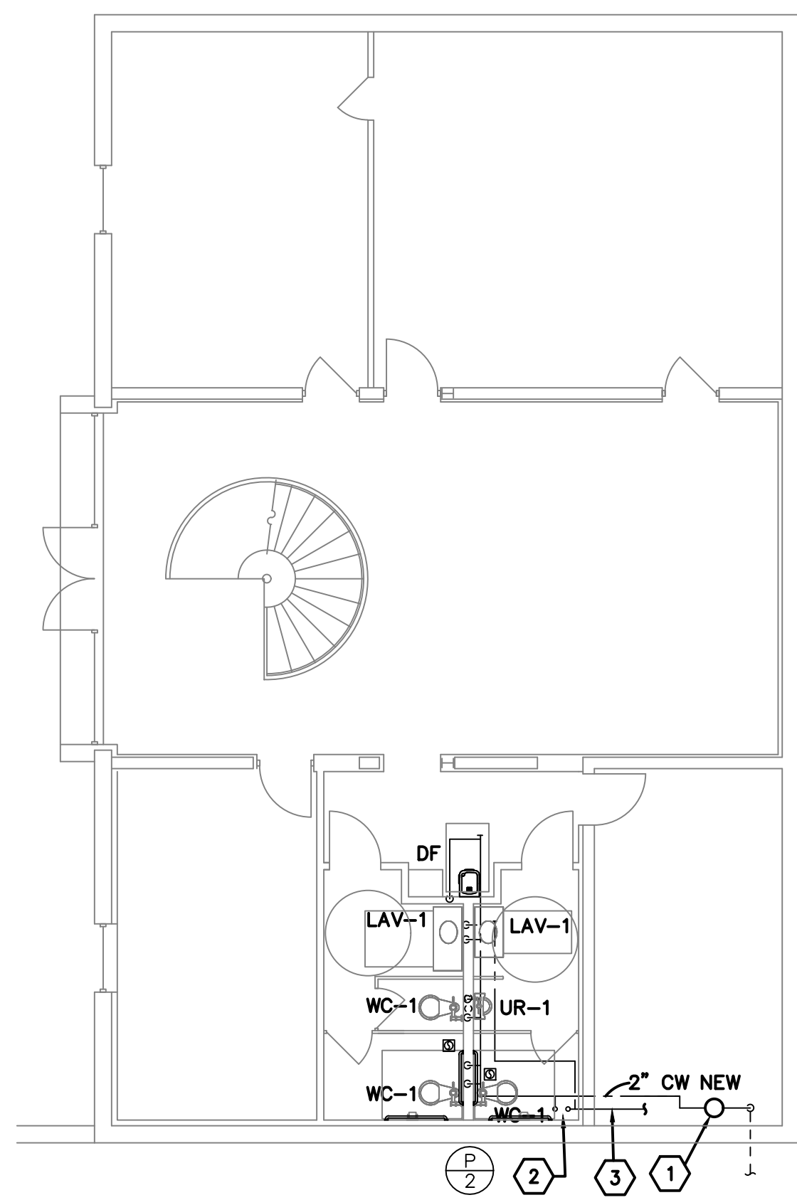
LOWER LEVEL WATER & VENT FLOOR PLAN SCALE: 1/8" = 1'-0"
