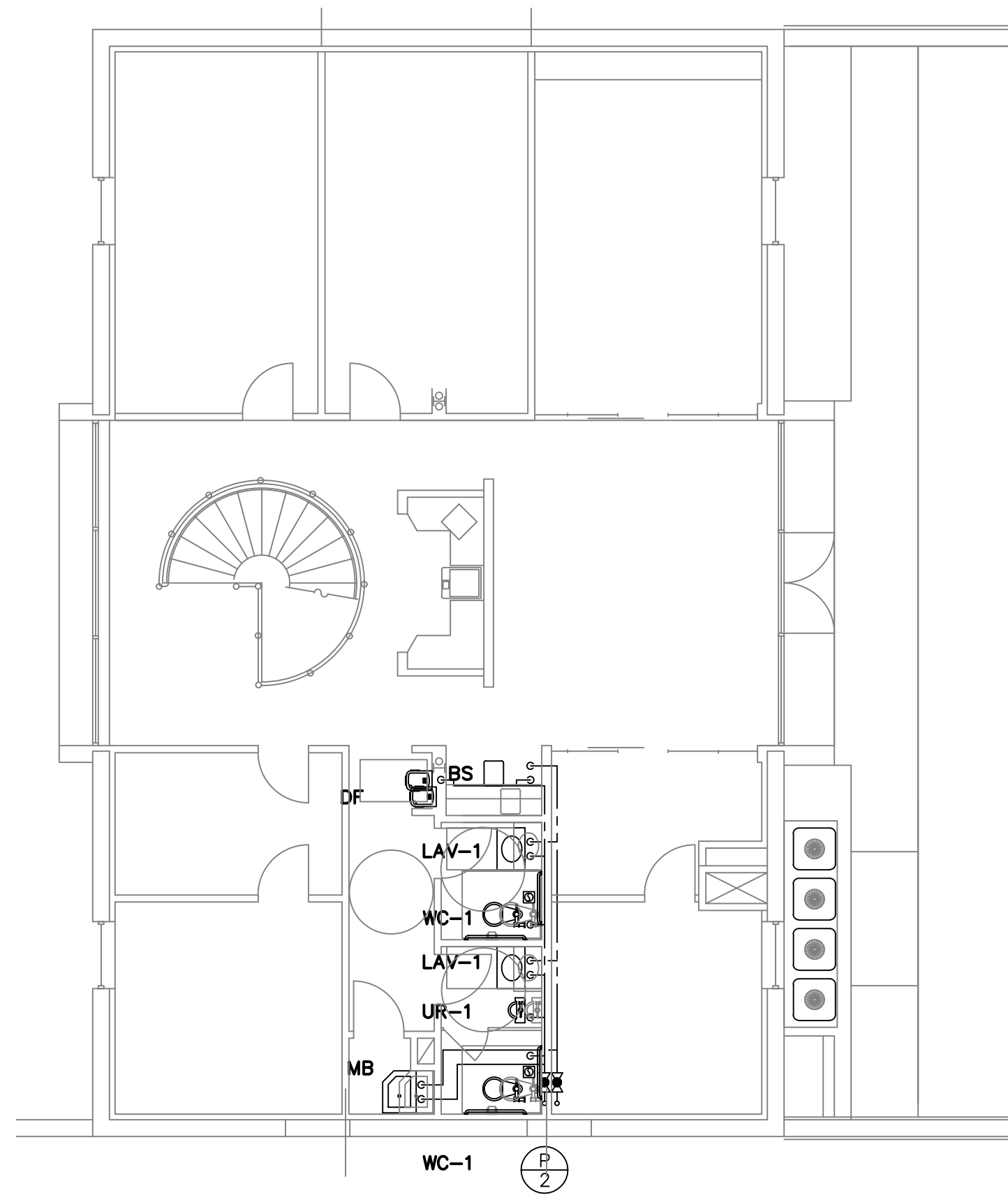
MAIN LEVEL WATER & VENT FLOOR PLAN SCALE: 1/8" = 1'-0"
