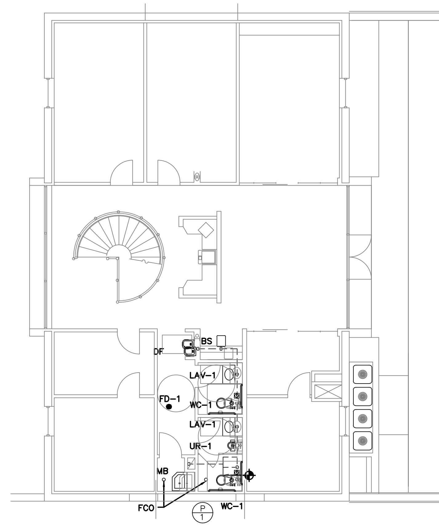
MAIN LEVEL WASTE FLOOR PLAN SCALE: 1/8" = 1'-0"
